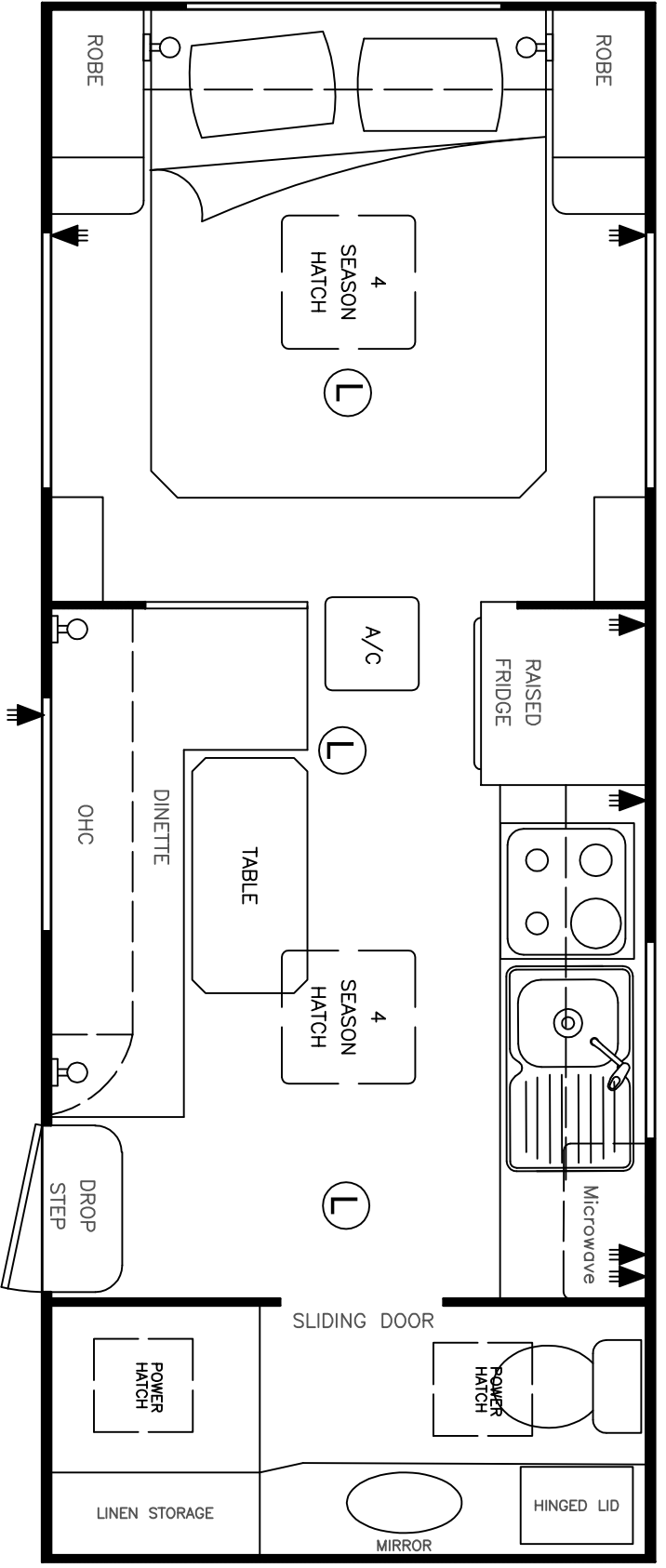
FLOOR PLAN Elegance 19'6"X7'8"
