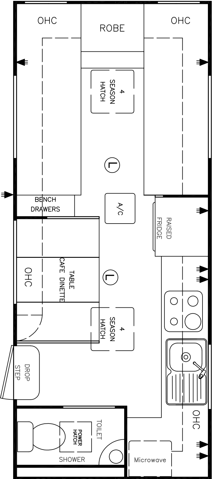
FLOOR PLAN Elegance 18'6"X7'8"
